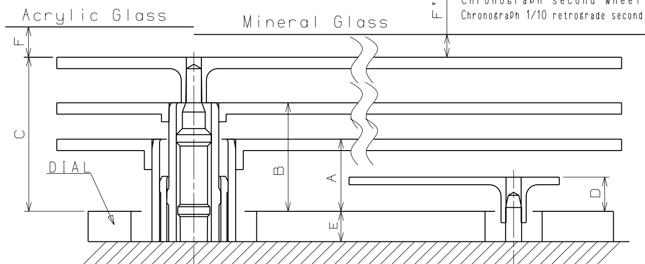
Chronograph second wheel
